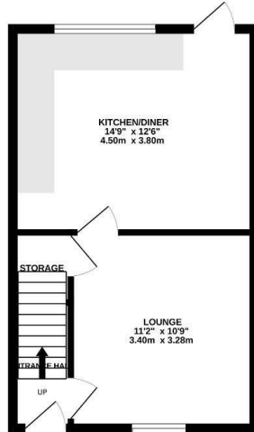
GROUND FLOOR 362 sq.ft. (33.6 sq.m.) approx.
